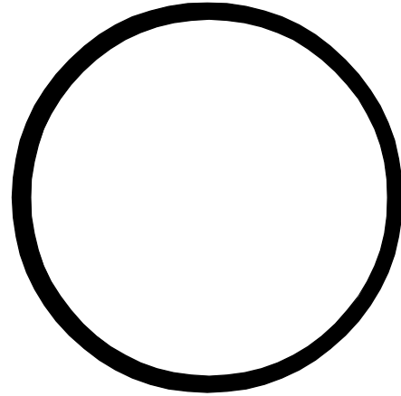
Cat. No. 00-4018-31 2.062 I.D. x 2.250 O.D. x 0.103 EP
