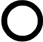
Cat. No. 00-4497-71 0.562 I.D. x 0.750 O.D. x 0.093 HYPALON CHEMICAL FEEDER Anit-Siphon Valve
