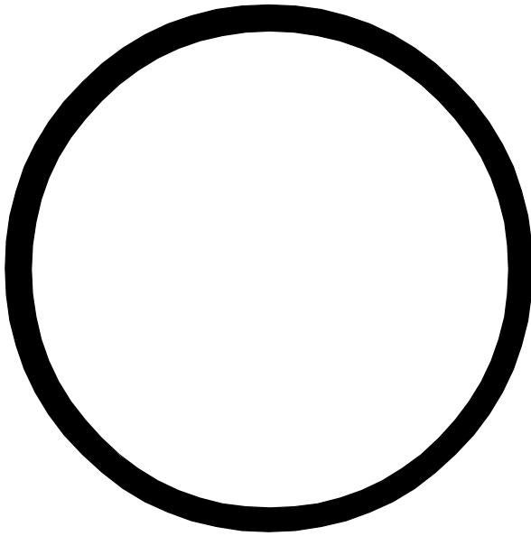
Cat. No. 00-4018-62 2.761 I.D. x 3.047 O.D. x 0.143 1989-Present HI-FLO ® 3 Regeneration Port
