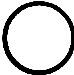
Cat. No. 01-0015-54 1.181 I.D. x 1.338 O.D. x 0.078 BUNA-N 1993-Present CULLIGAN ® MARK 1000 Meter, Inlet/Outlet Coupling
