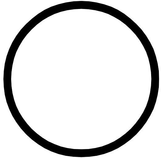
Cat. No. 01-0016-11 2.375 I.D. x 2.625 O.D. x 0.125 EPT
